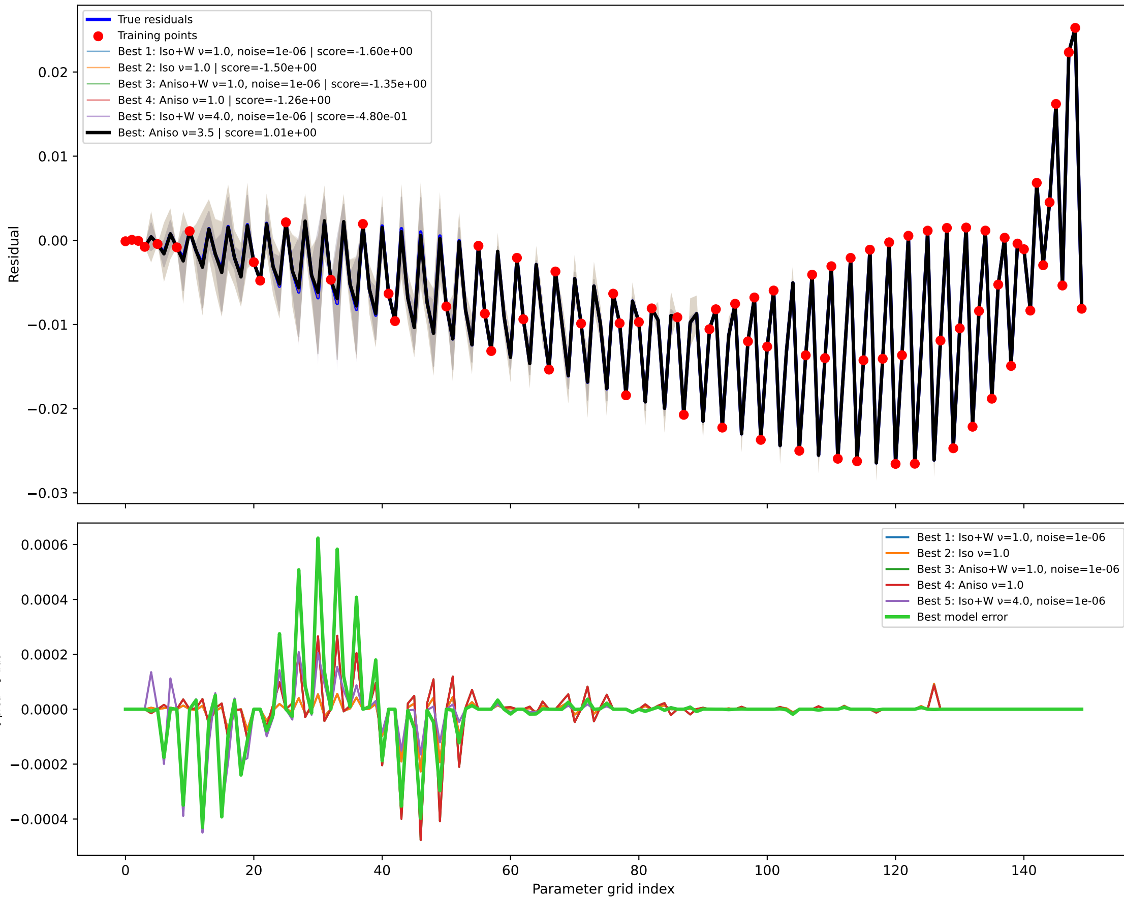
GPR kernel comparison node=0 RMSE=1.244e-04, train RMSE=3.166e-11
